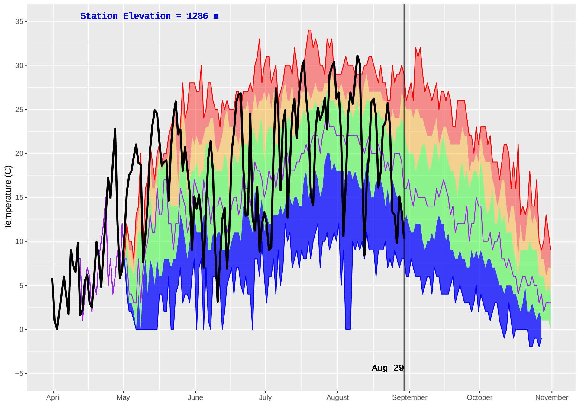
CURWEN CREEK (352) : Historical (1979–2016) and Current (2018) Daily Temperature
